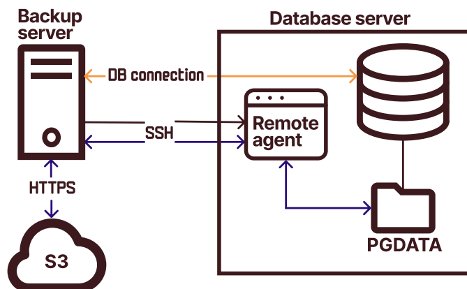
Figure H.1. pg_probackup setup with a remote agent and S3
