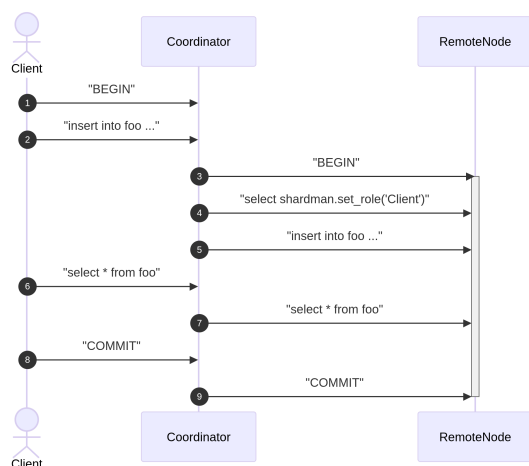
Figure 53.5. Connection Flow Chart
